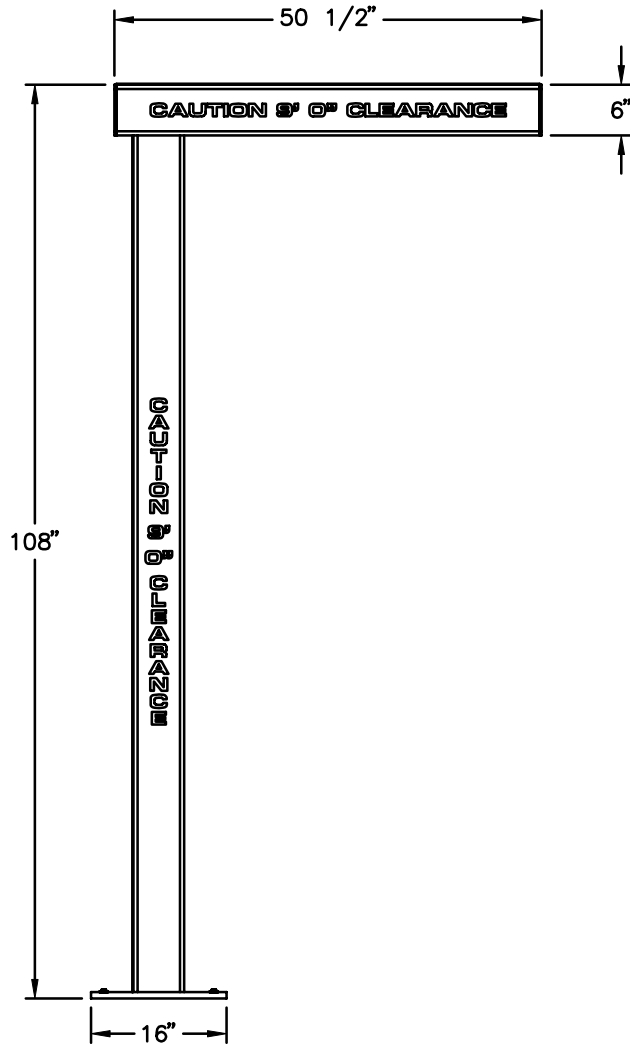
FRONT VIEW
