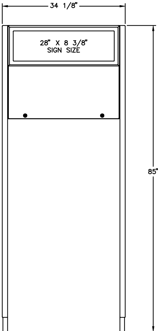
FRONT VIEW
