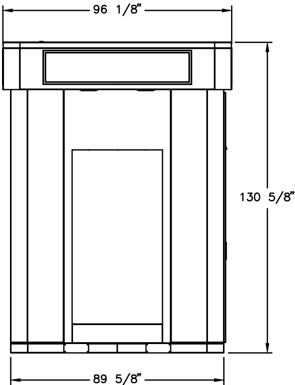
FRONT VIEW
