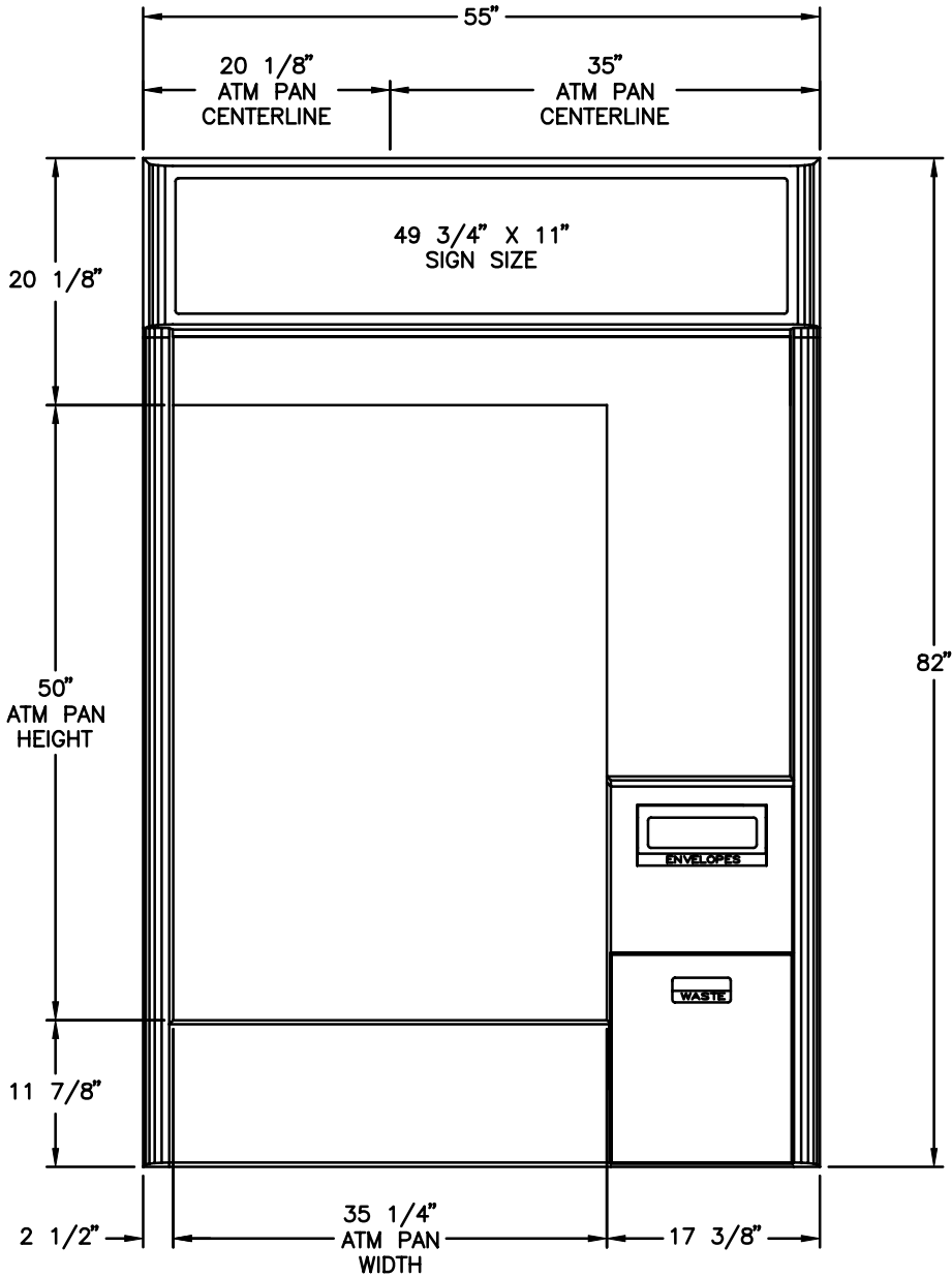
FRONT VIEW
